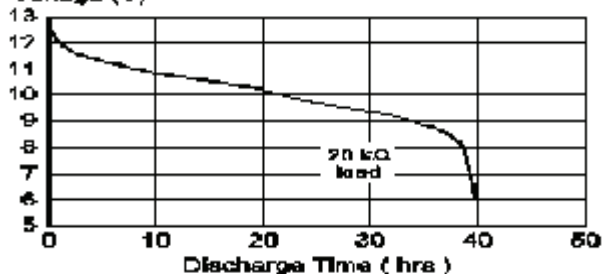
Normal Rate Discharge Voltage (V)
